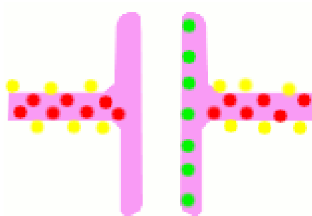
FIG. 4. Action potential of sodium/ potassium pump.
